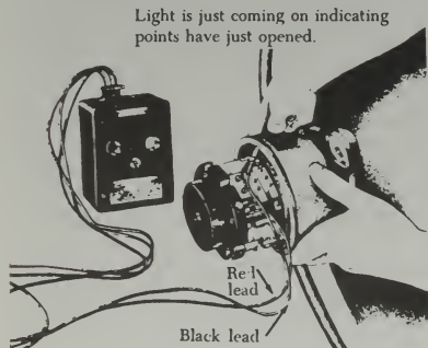
FIGURE 4-49. Timing the low-tension distributor to the engine.
